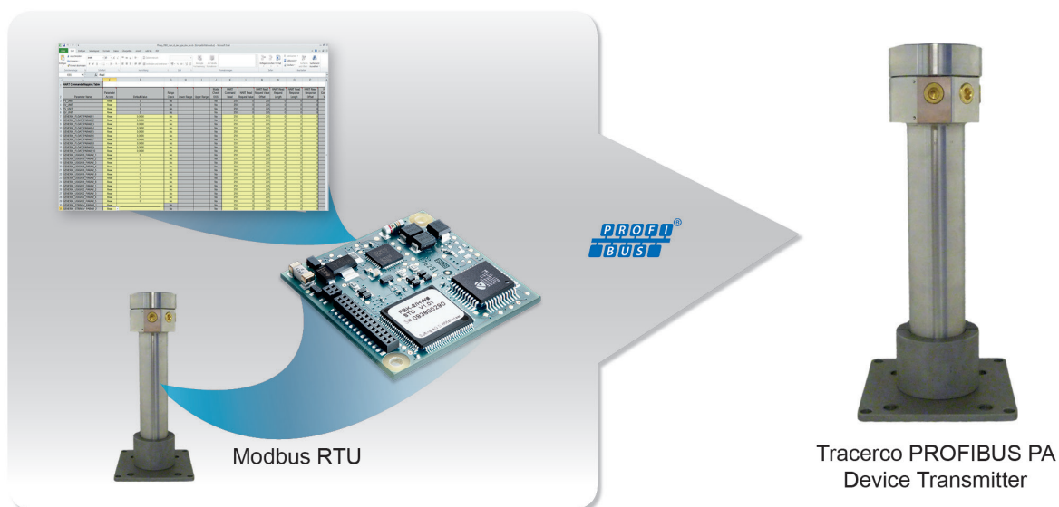
Implementation of Tracerco's PROFIBUS PA Interface by Configuring PAeasy Firmware
