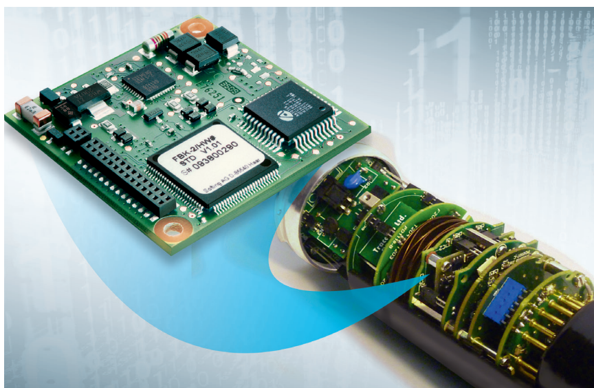
Tracerco Hyperion™ Density Transmitter Supporting PROFIBUS PA Communication
